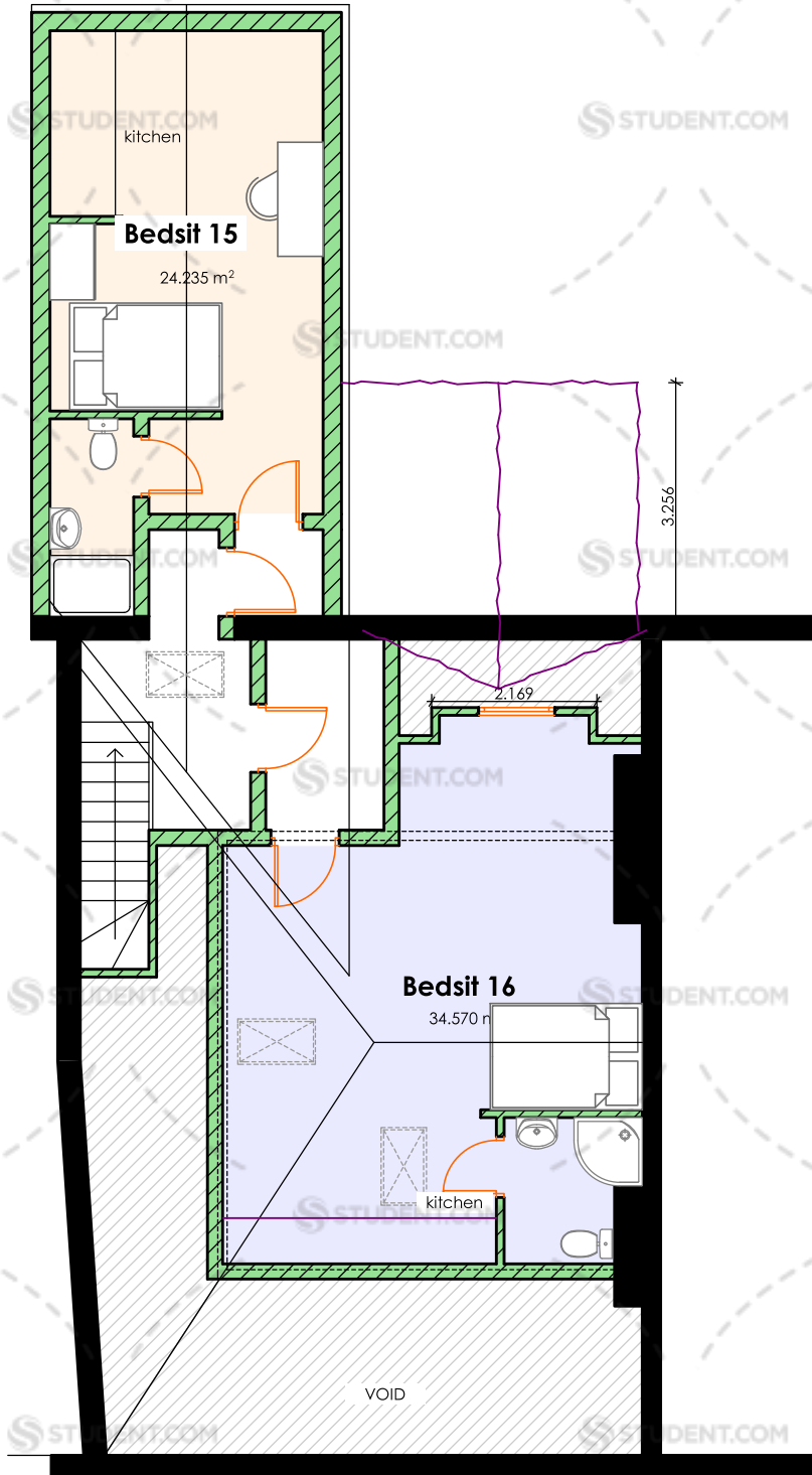
Proposed Loft Plan @ 1:100
